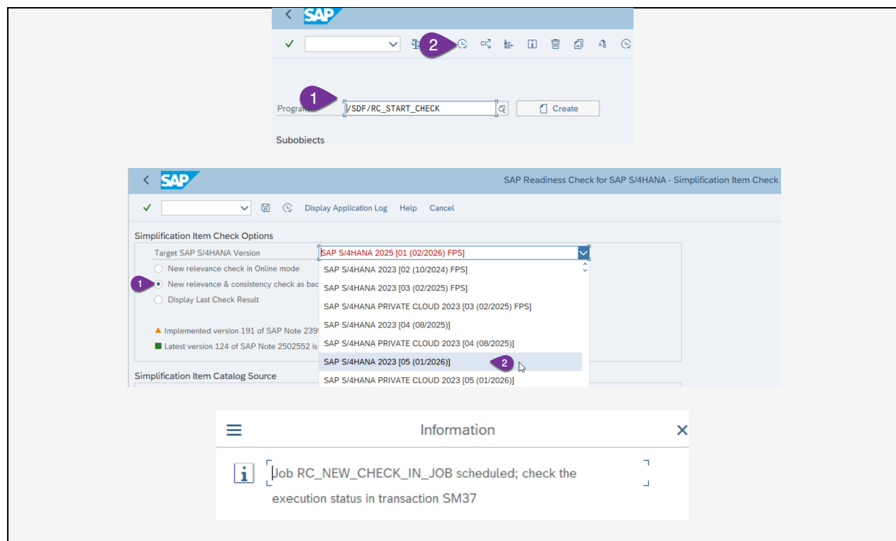
/SDF/RC_START_CHECK selection screen — target version and options configured
